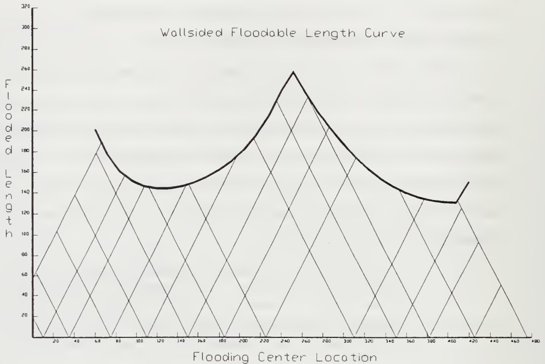
Figure 6. Wallsided Floodable Length Curve
